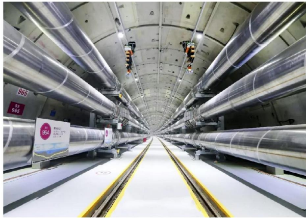
1100kV GIL in Sutong project, Jiangsu Province
