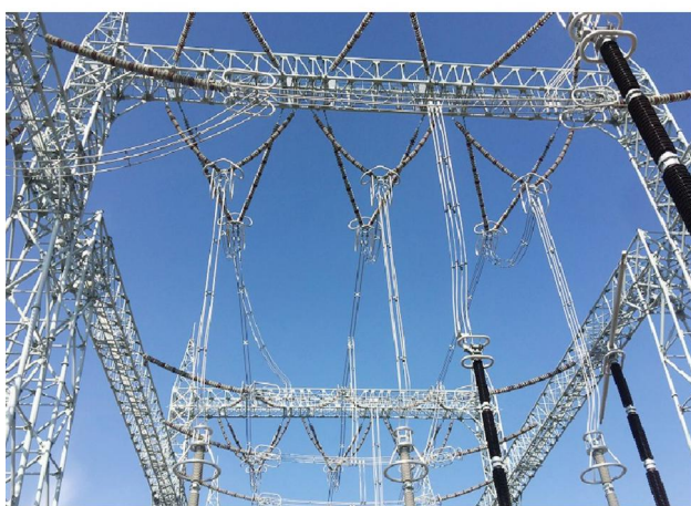
± 1100kV Changji converter station DC station electric power fittings
