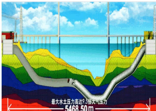
Sketch map : 1100kV GIL project through the Yangtze river
